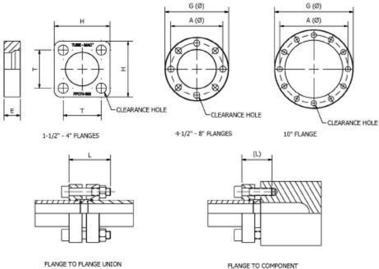
Retain Ring Flange Dimensions, Metric
