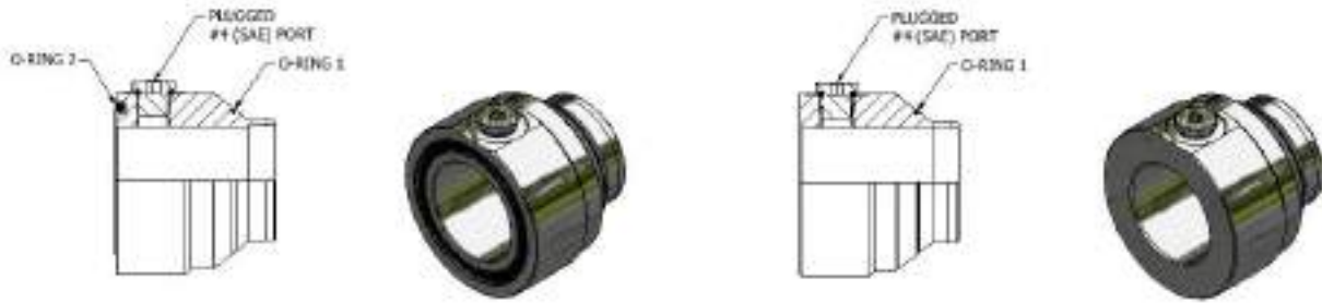
COP and CFP - Cone Inserts with Pilot Port for Flare Flange Connections, NPS
